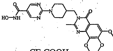
.CF 3 COOH compound 8
